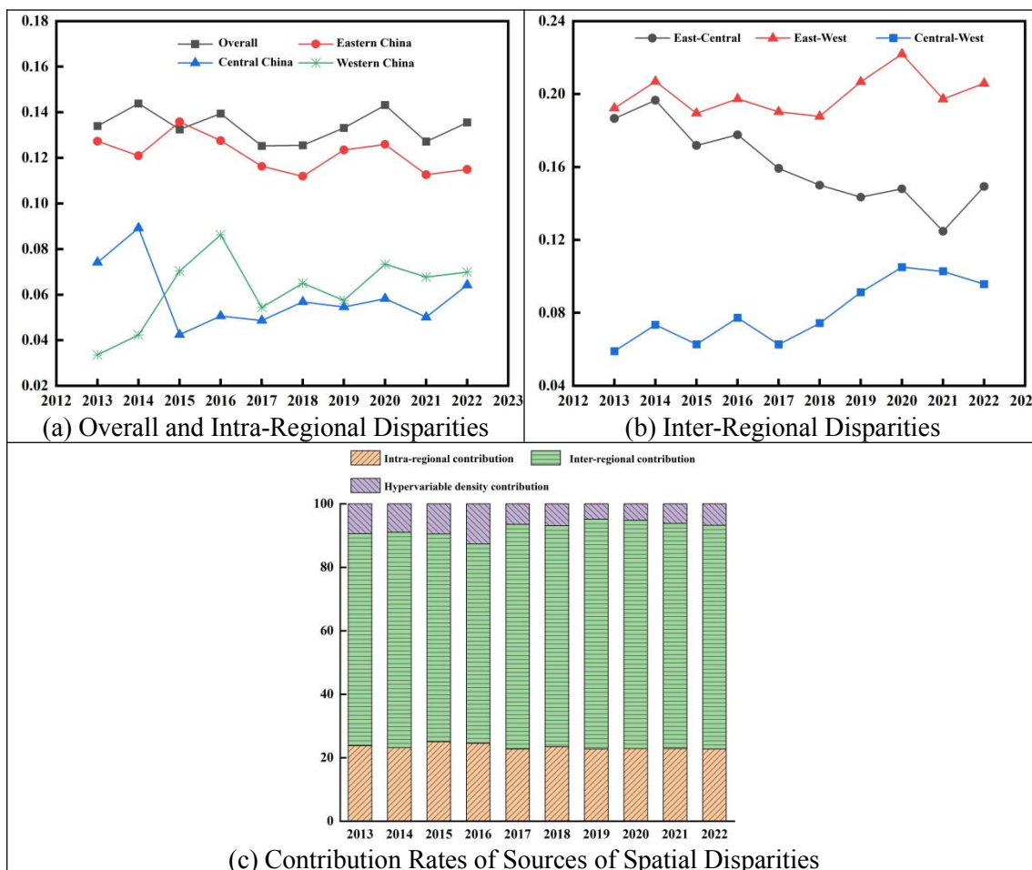
Figure 2. Temporal evolution and decomposition of the Gini coefficient
