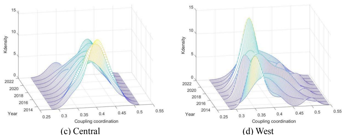
Figure 3. Kernel density estimation
